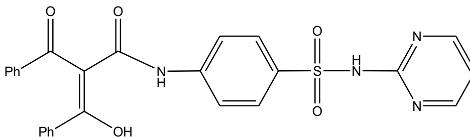
Figure 1. Structure of the N-carboxamide ligand
