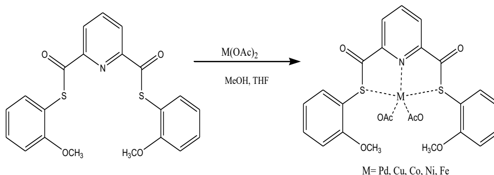
Figure1. Synthesis of thioether ligand
